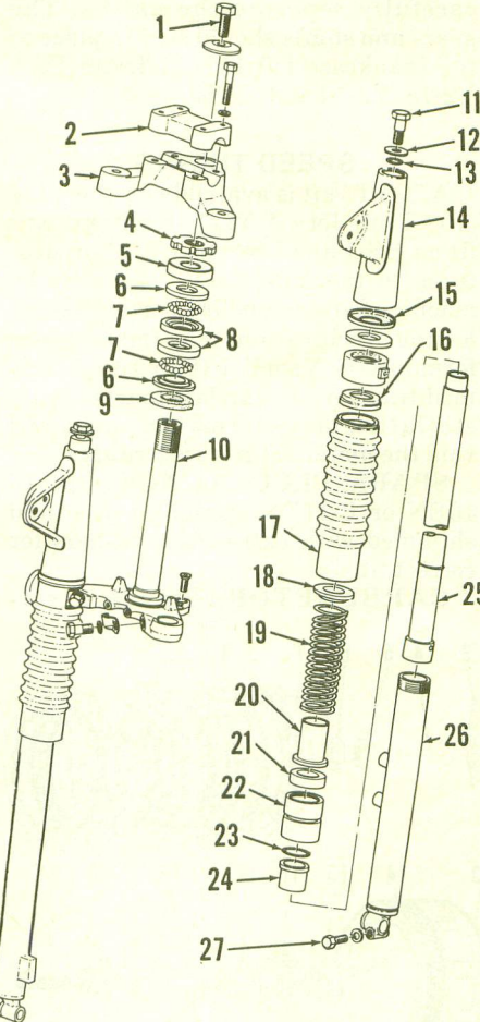
Fig. Y2-12—Exploded view of front fork assembly used on HS-1. Forks used on other models are similar.
