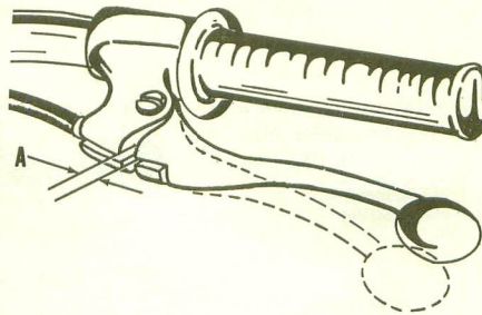
Fig. Y5-9—The clutch hand lever should have 2-3MM free play at (A).
