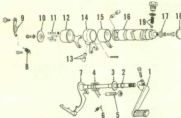
Fig. Y4-19—Exploded view of the clutch assembly. Parts (20 thru 24) are located in left cover.
