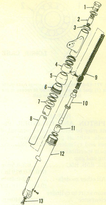
Fig. Y11-10—Exploded view of model DS7, R5, R5B and R5C front suspension unit.
