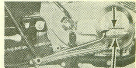
Fig. 2-42—Rear brake pedal should normally lock rear wheel when compressed approximately \frac{7}{8} inch.
