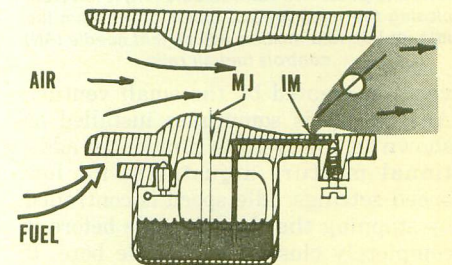
Fig. 1-7—As disc type throttle valve is moved toward the closed position, vacuum at the main jet (MJ) may not be enough to draw fuel into the passing air and an intermediate jet (IM) is provided.
