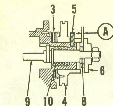
Fig. Y7-7—Clearance (A) is adjusted by varying shims (8).
